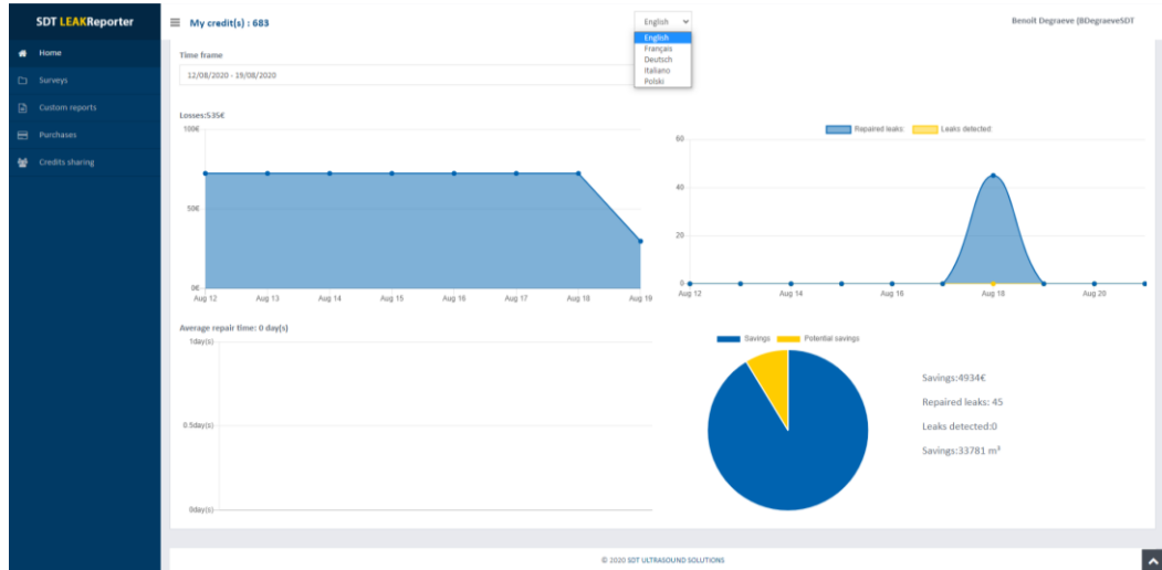
LEAKReporter App
