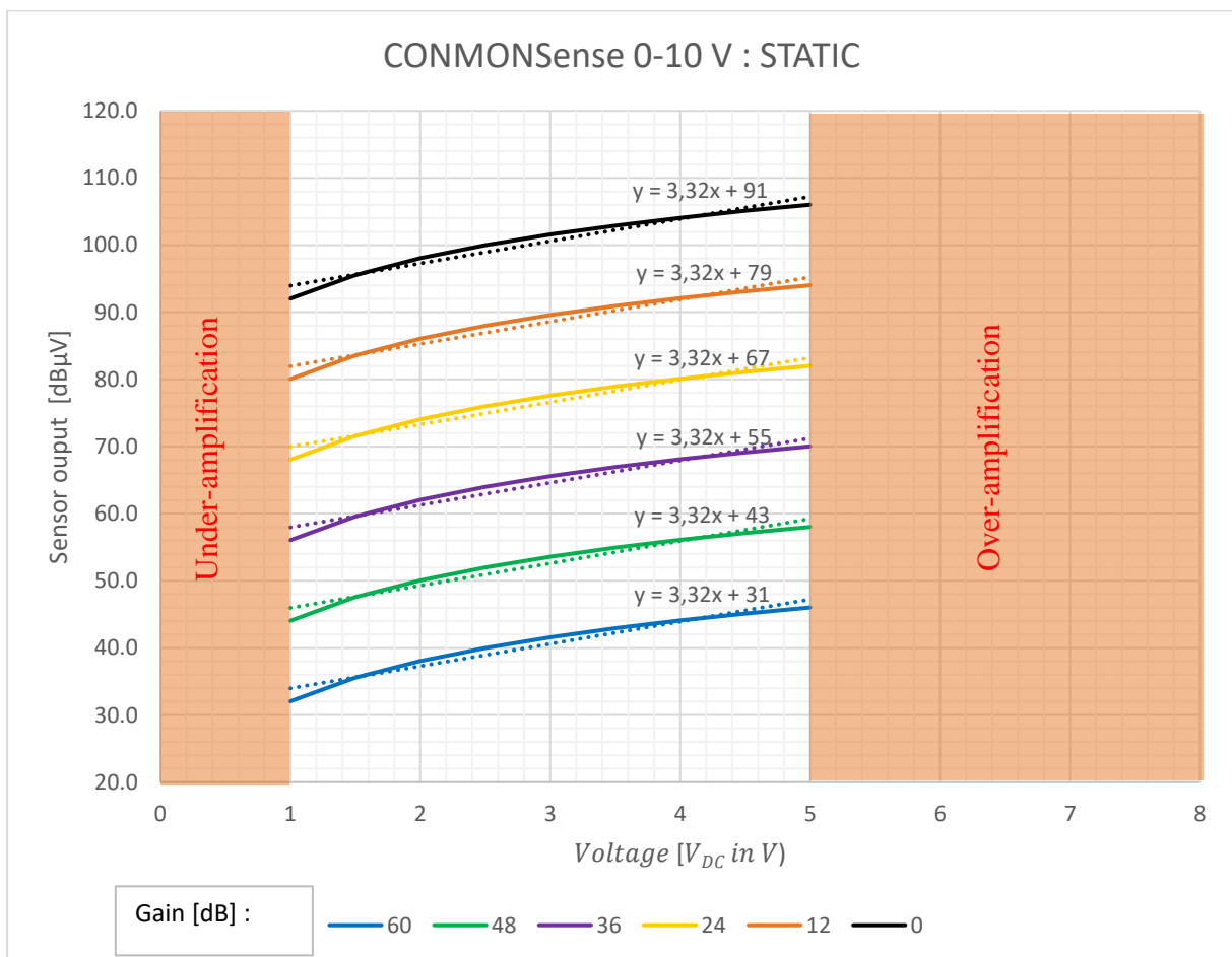
Figure 1: Sensor signal in dBμV vs Voltage, for each gain
