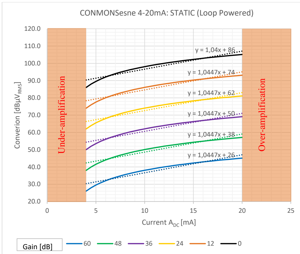
Figure 2: Sensor signal in dBµV vs Current, for each gain (loop powered)
