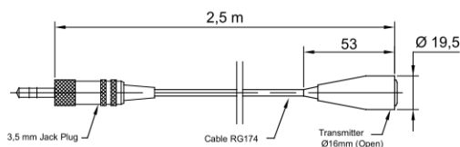
Figure2: Closed transducer 18mm
